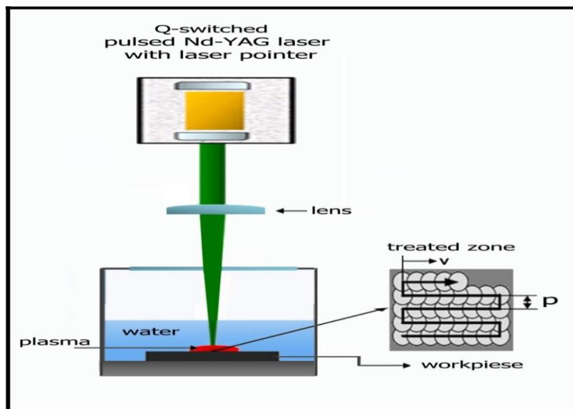
Figure 3. Laser shock peening technique.
