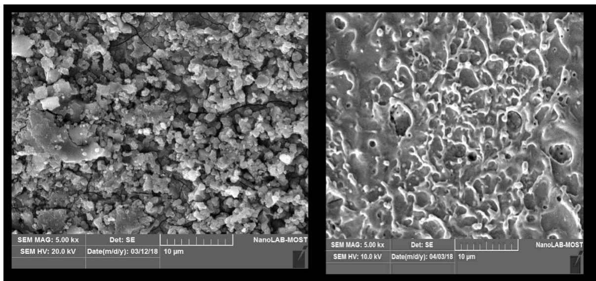
Figure 4. SEM graphs of corrosion samples (left: without nanocoating) & with nanocoating.
