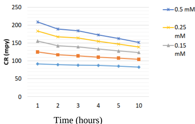
Figure 2. Corrosion rate per year as a function of time period with organic inhibitor for different acid molarity.
