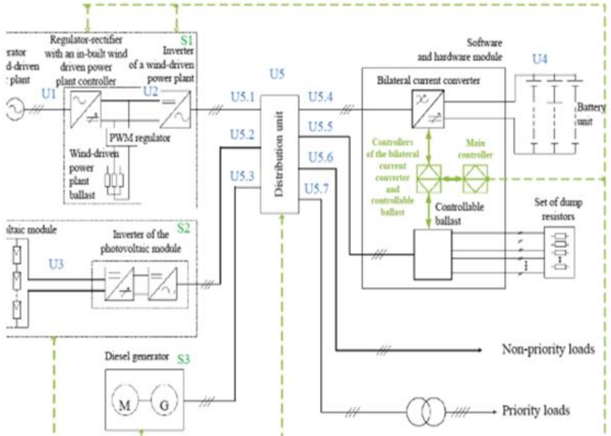
Fig. 2. General structural diagram of an off-grid power supply facility, comprising renewable energy sources and controlled by an intelligent power conversion/control/distribution system: — high-speed communication interface;
